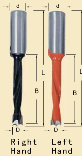
77MM Length, 10MM x 27MM Shank Do not use in portable drills or routers.
