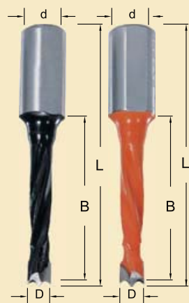
4-Flute High Performance Brad Point Boring Bits 10mm Ø20mm Shank High performance carbide for ultra long lasting applications.
