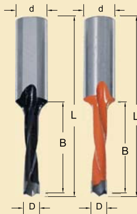
High Performance Brad Point Boring Bits High performance carbide for ultra long lasting applications.
